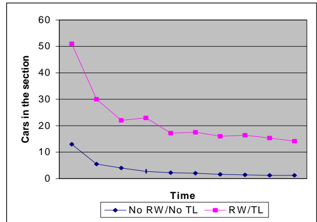
Figure 11: Execution Results Adding Traffic Lights.
