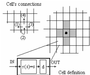
Figure 1. Definition of a Cell-DEVS Model
