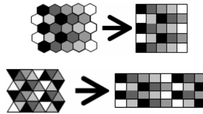
Figure 2. Shift mapping to the square lattice.
