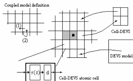
Figure 1. Informal definition of Cell-DEVS.
